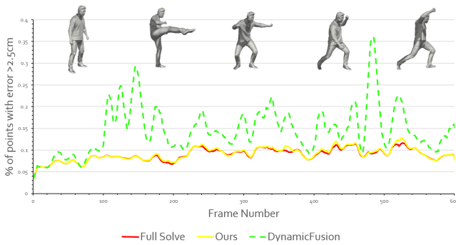
Figure 4: Solver convergence over a sequence for a fixed number of iterations: Green dashed line demonstrates an approximate evaluation of \mathbf{J}^\top \mathbf{J} . Red line shows an exact Cholesky solve. Our method is shown in yellow and shows similar convergence behavior as the exact method, with improvements over approximate approaches.
