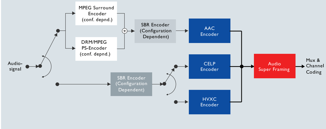
Figure 6.2.1a: DRM audio coding
