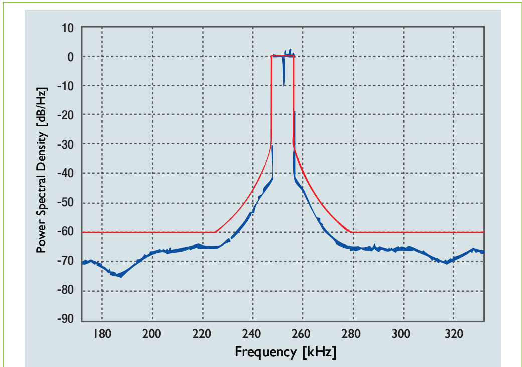
Figure 9.2.7: DRM LF TX Spectrum
