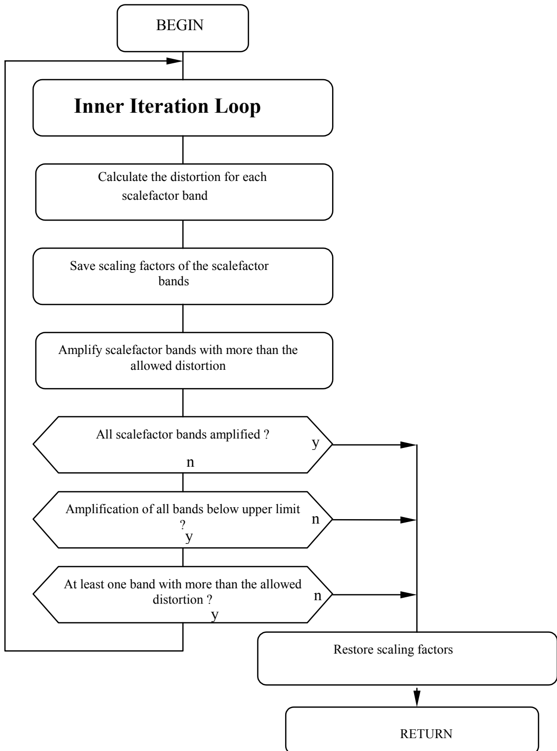
Figure C.7 — AAC outer iteration loop
